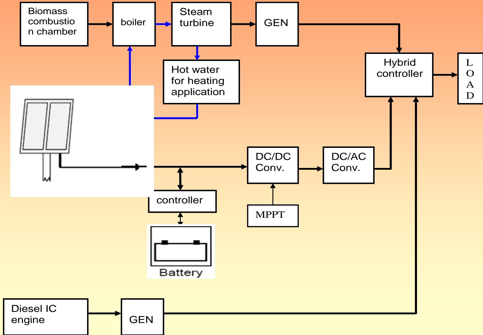
Block diagram of biomass-PV-Diesel Hybrid System
