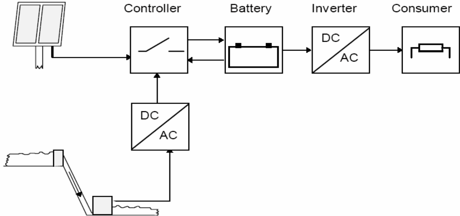
Schematic diagram of a typical hybrid energy system containing solar and hydro sources.
