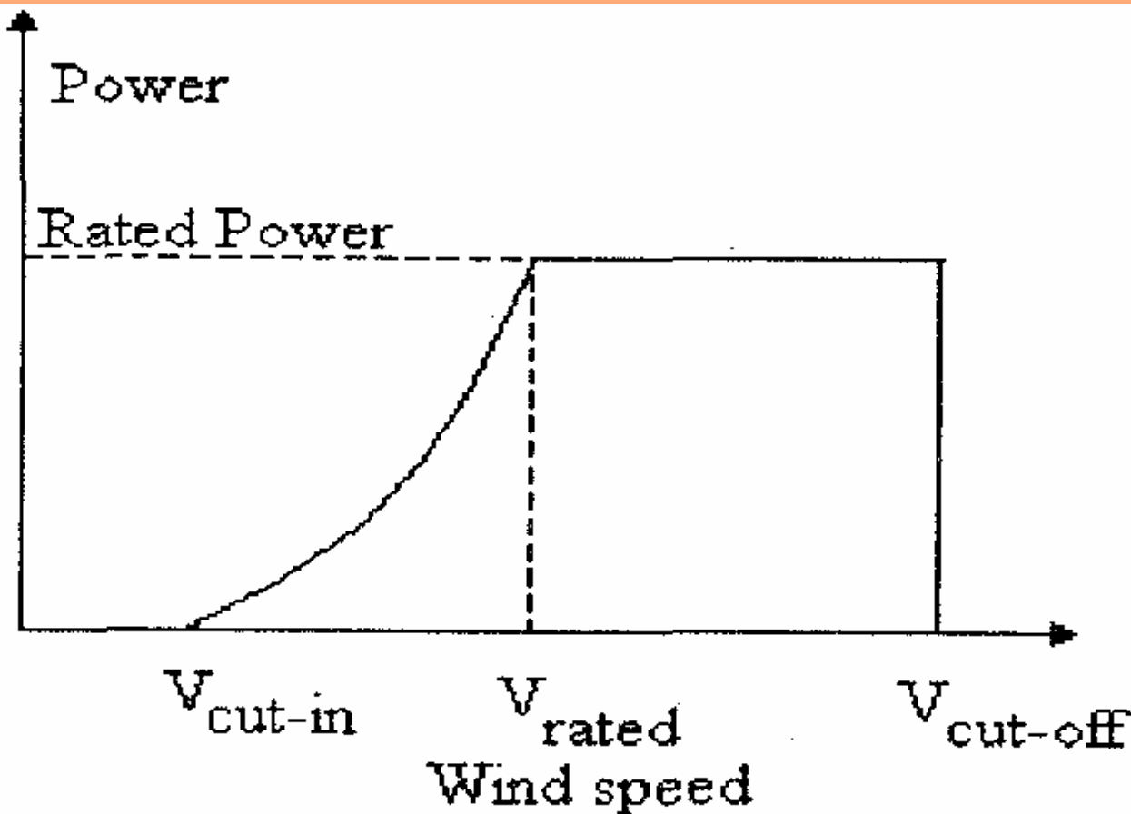
Power wind Speed Characteristic.
