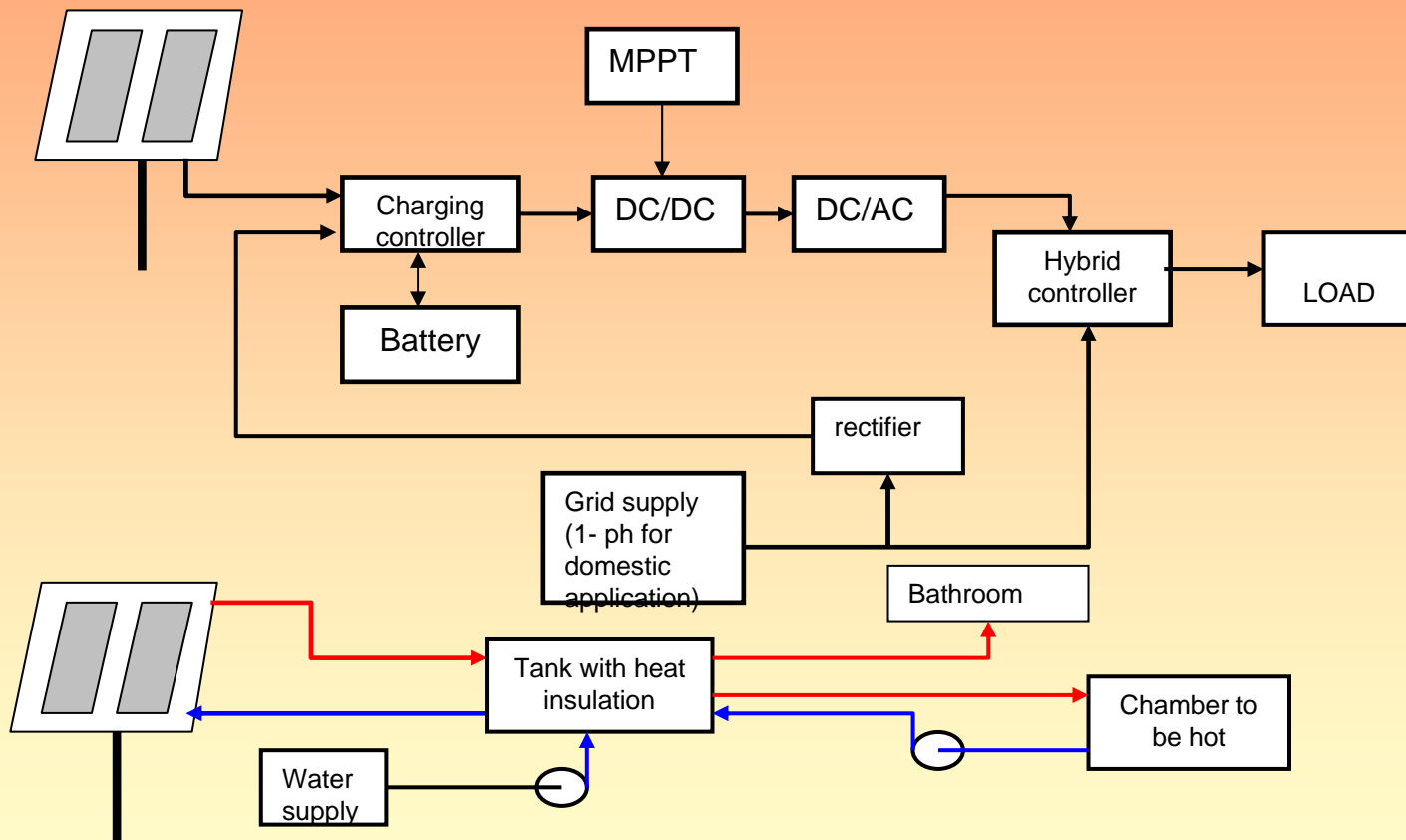
Block diagram of PV-grid connected-solar thermal Hybrid system
