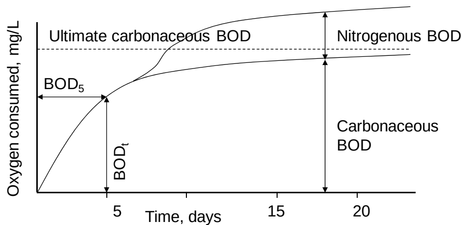
Figure 11.2 Nitrification during BOD test
