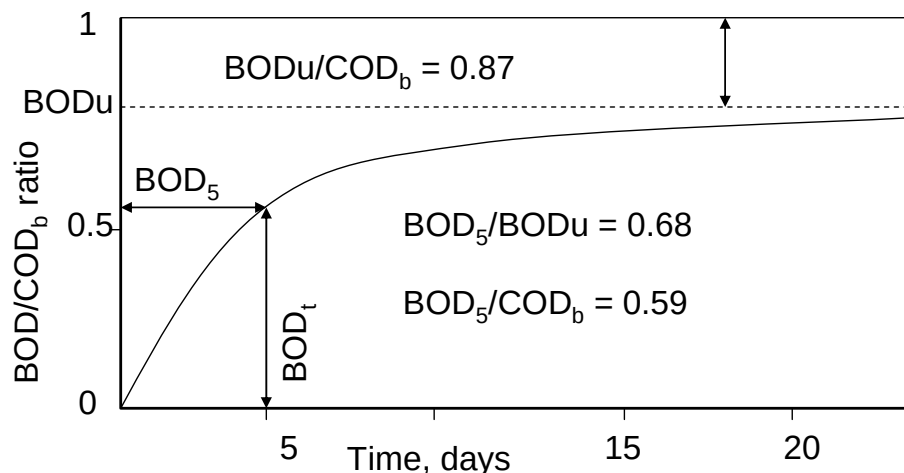
Figure 11.3 Correlation between BOD and COD for sewage at 20°C incubation and k = 0.23 per day.
